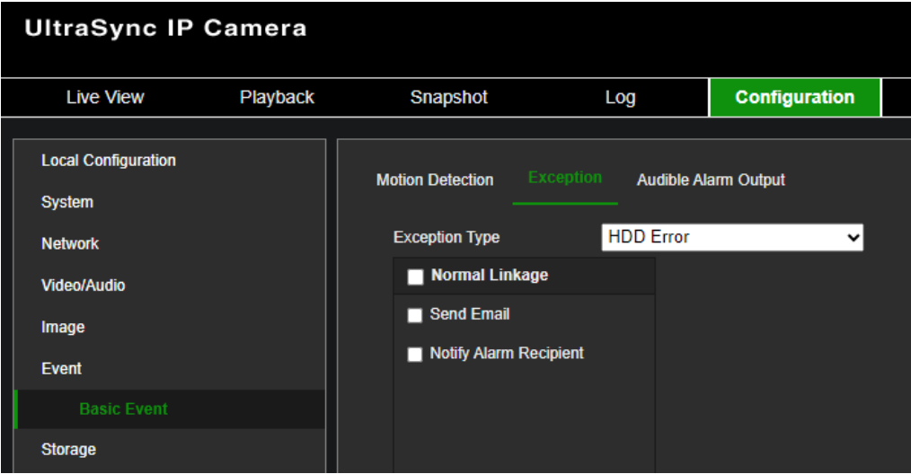
Figure 7: Exception window
