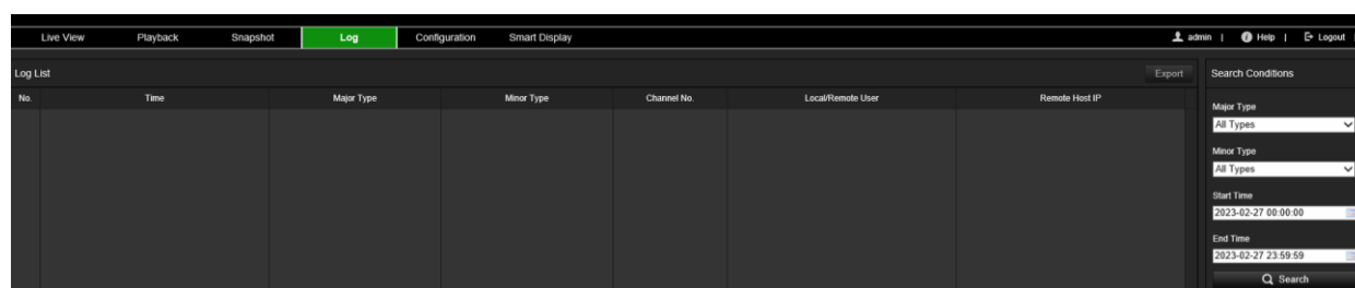
Figure 13: Log window
