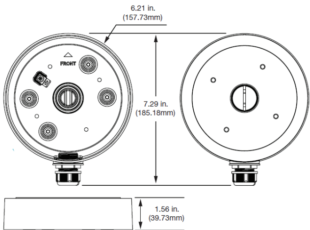
TVP-CBB TruVision Compact PTZ Back Box
