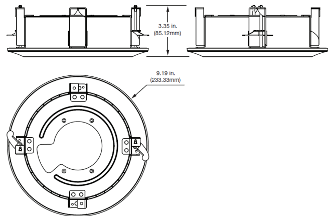
TVP-CFM TruVision Compact PTZ Flush Mount
